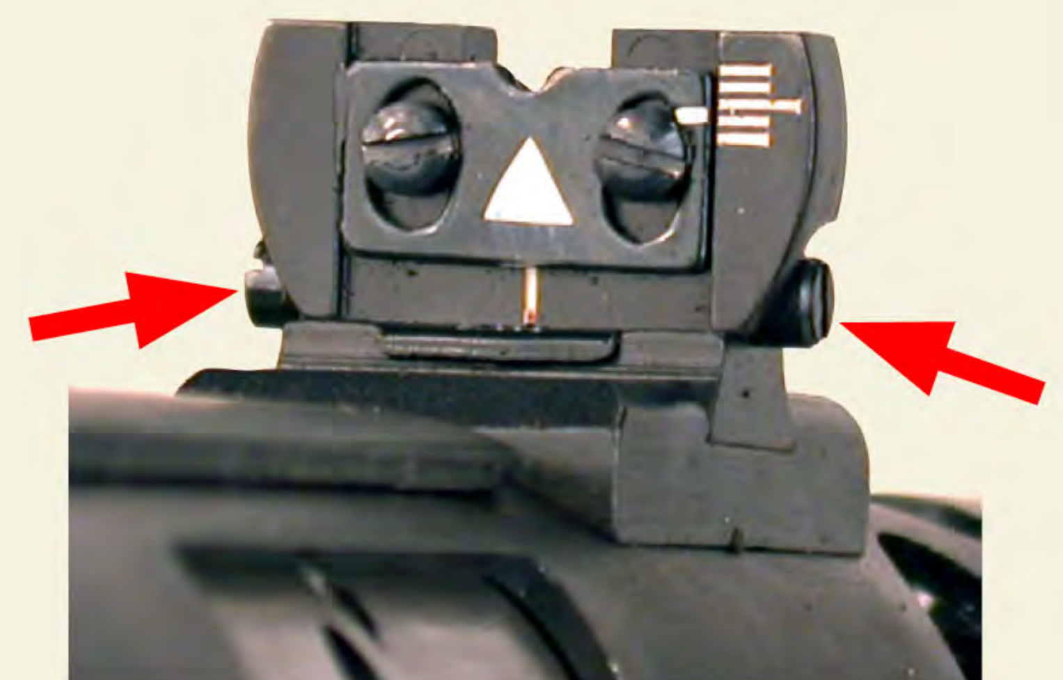
Right: The fold-down rear sight was rudimentary yet efficient. It was windage adjustable by using a small screwdriver in the slots (arrows).
