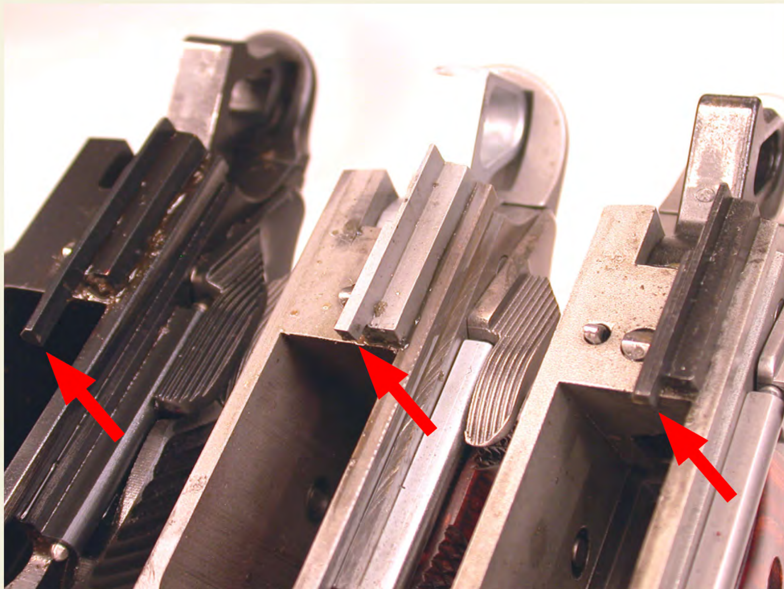
Above: The ejector on our STI Duty One, left and detail, below , was much longer than those found on either the Kimber, right, or Springfield Armory pistol, center. After suffering malfunctions, we returned our Duty One to STI for warranty service.
